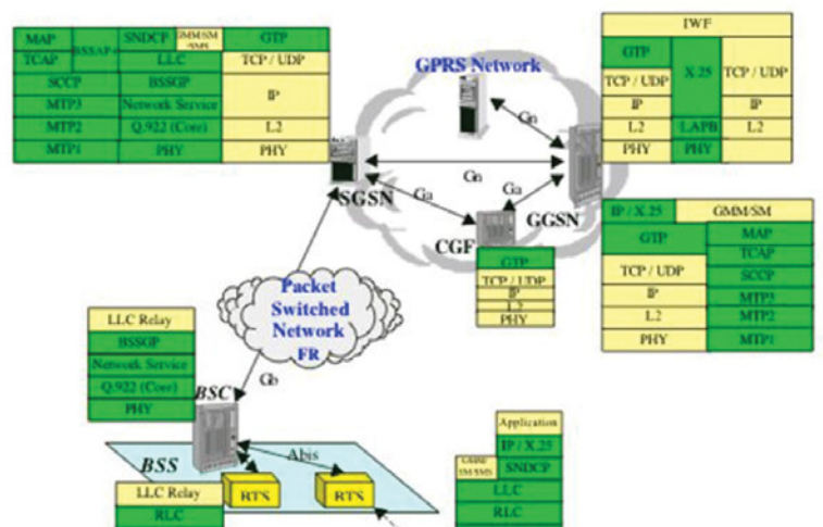
Figure 2. Protocols used in BTS, BSC, SGSN, GGSN, and mobile handsets
