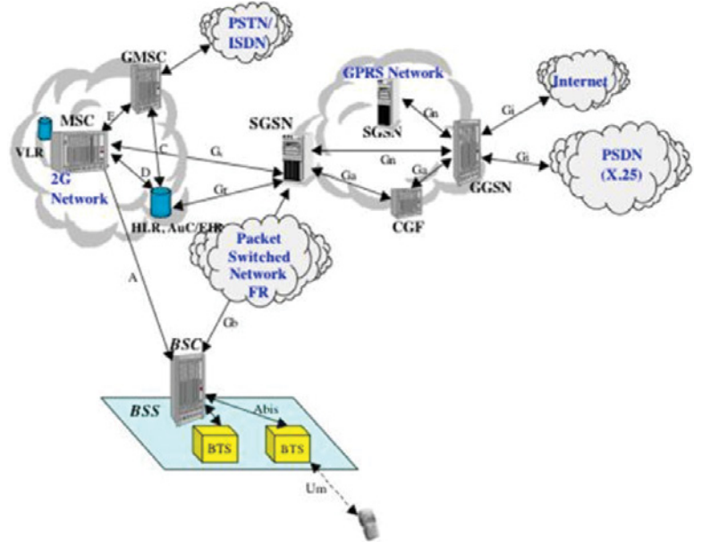
Figure 1. A GPRS Network
